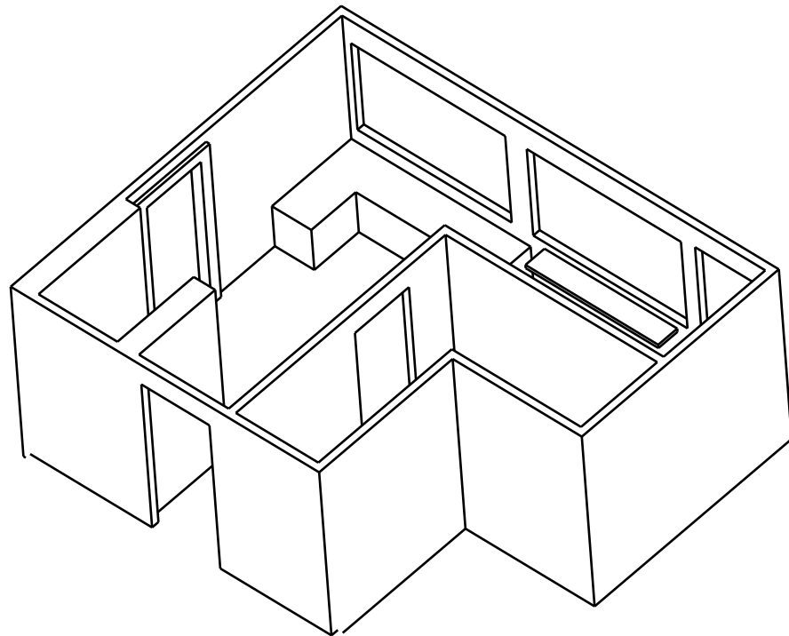
Isometric view Scale: 1:70
